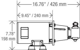
Feed Pump
